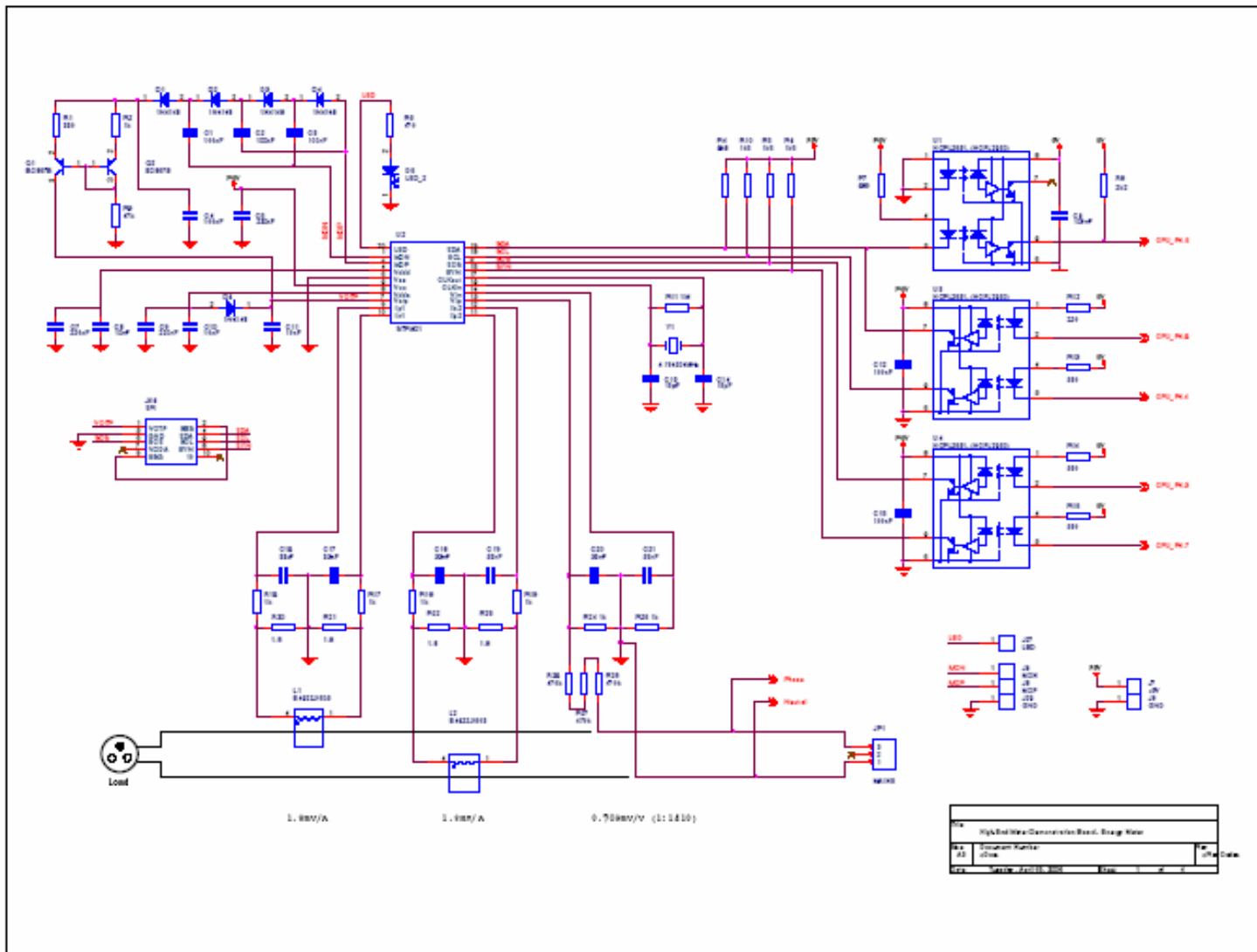
Figure 4: Energy meter section schematic
