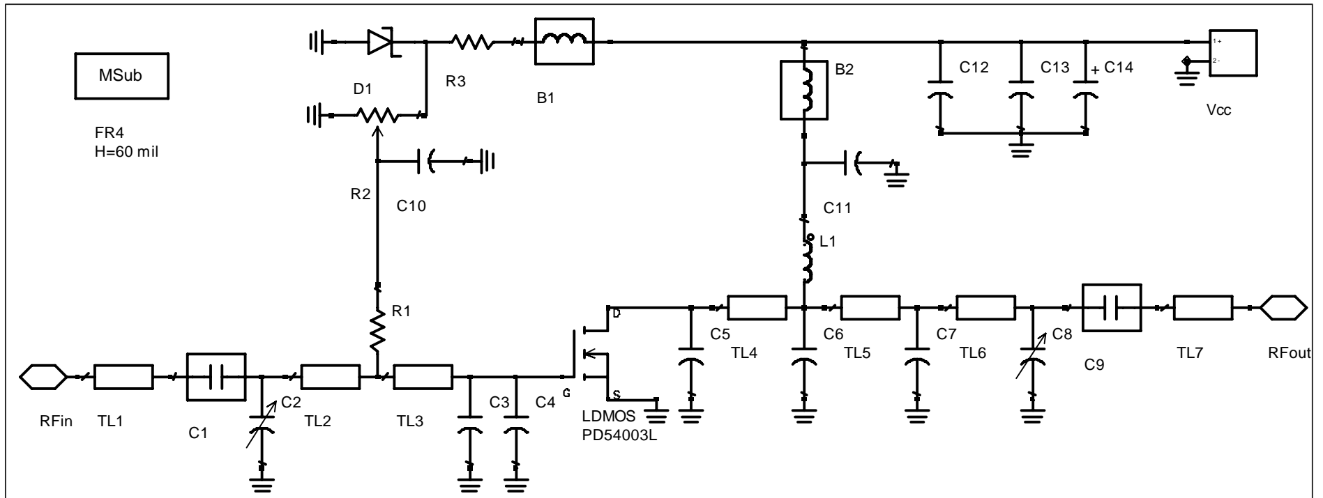
DB-54003L-880 schematic
