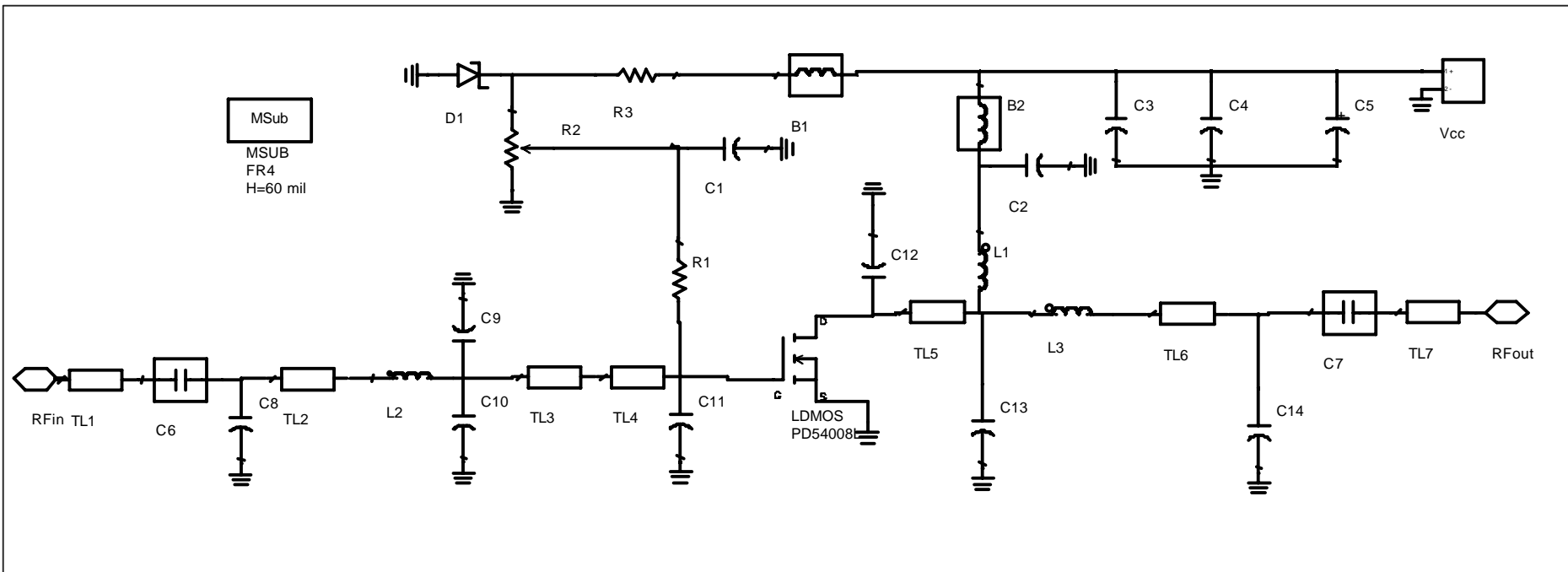
DB-54008L-830 schematic
