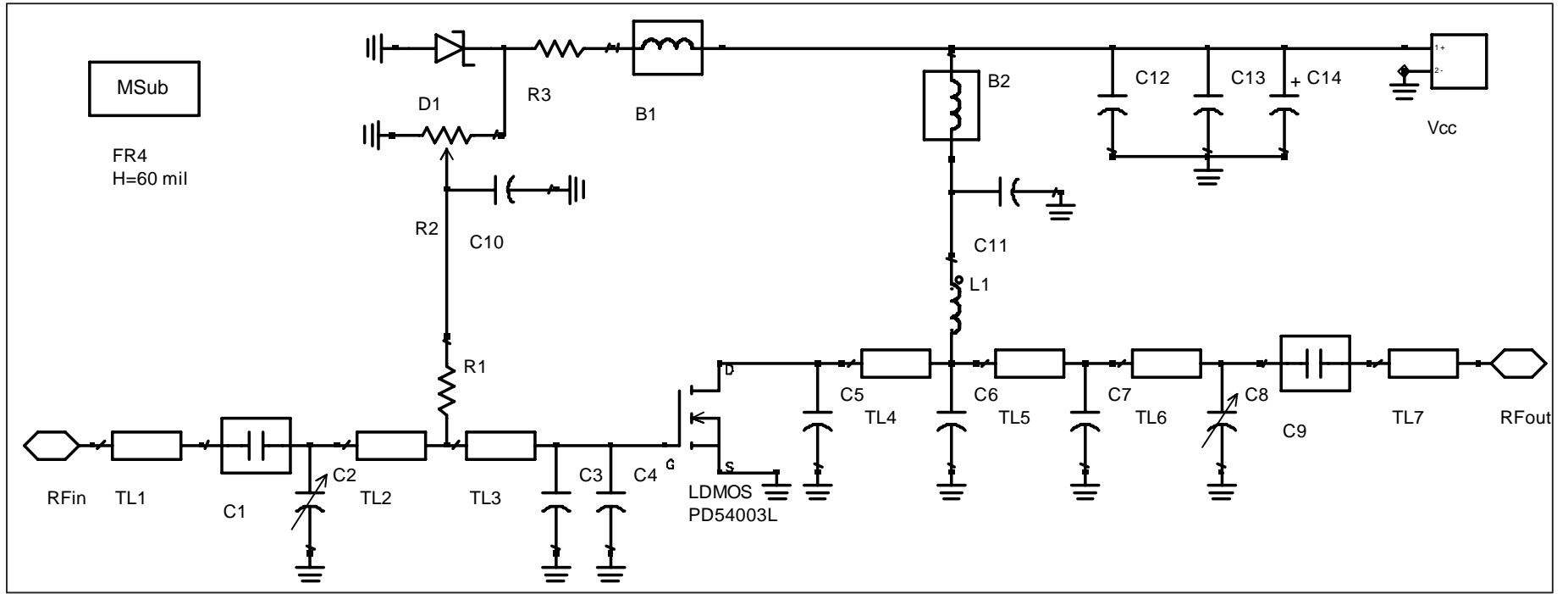
DB-55008L-880 schematic
