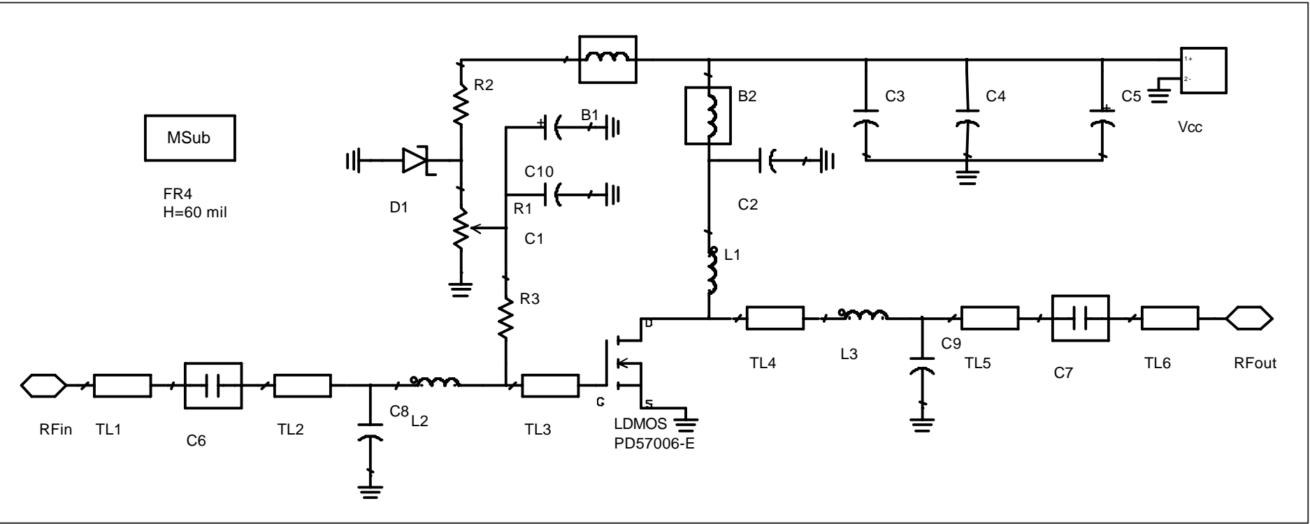
DB-57006-600 schematic
