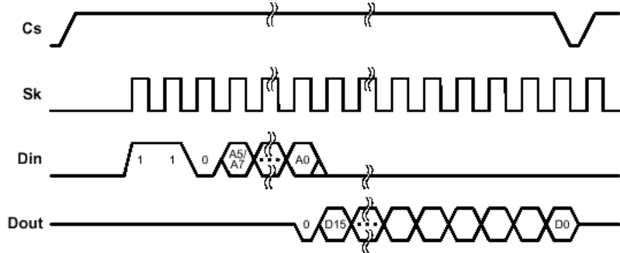
Figure 3. Read Operation
